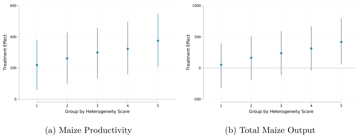
Figure 2: Sorted Group Average Treatment Effects, estimated with Neural Nets
